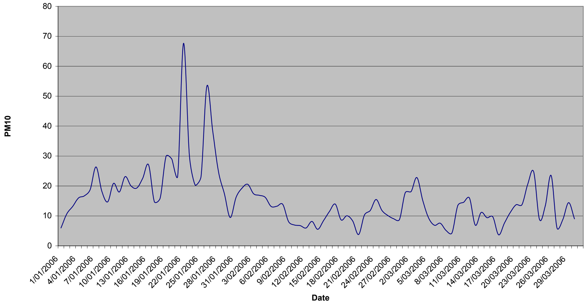
PM10 averaged over 24 Hrs 1/1/2006 to 31/3/2006
